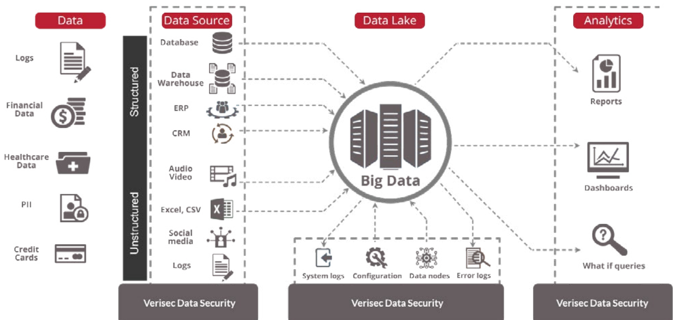
Verisec Transparent Encryption providing end-to-end data encryption, privileged user access control, and key management in a big data environment.
